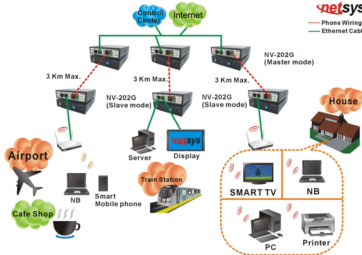
Figure 2.6 NV-202G point to point applications
