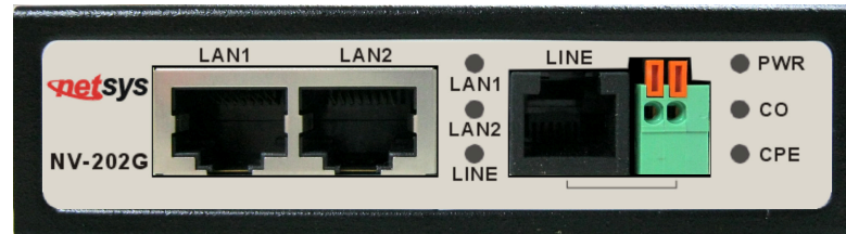
Figure 3.1 Front Panel
